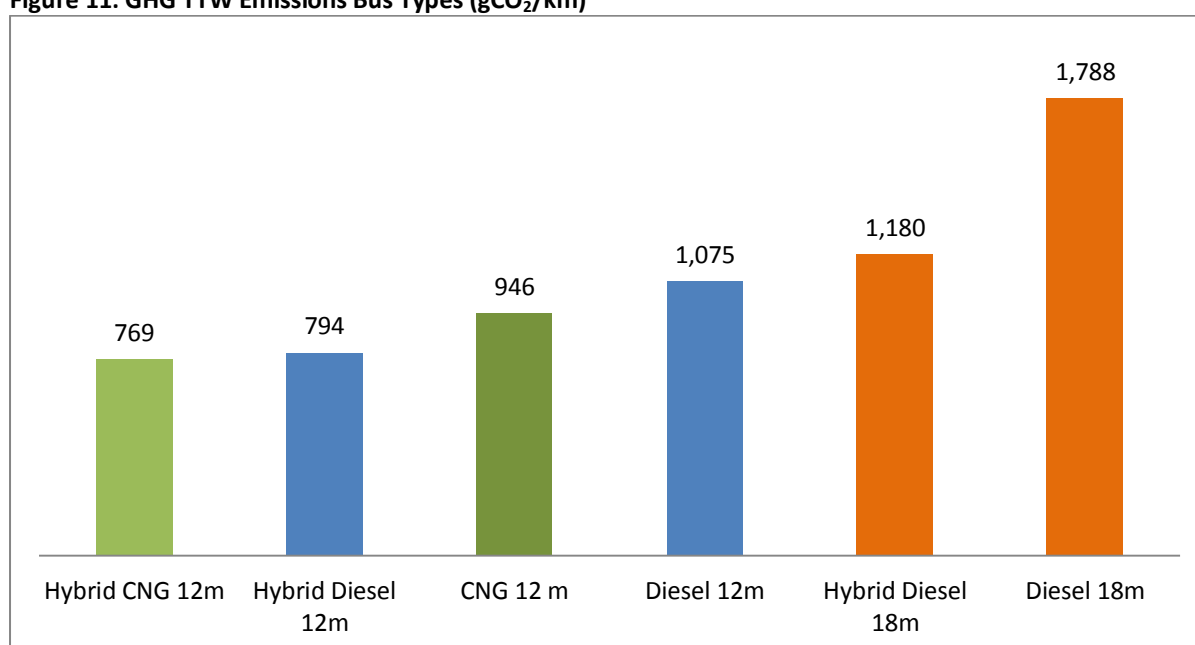
Figure 11: GHG TTW Emissions Bus Types (gCO 2 /km)
