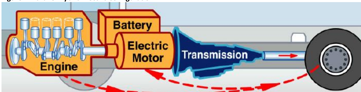
Figure 4: Parallel Hybrid Electric Configuration
