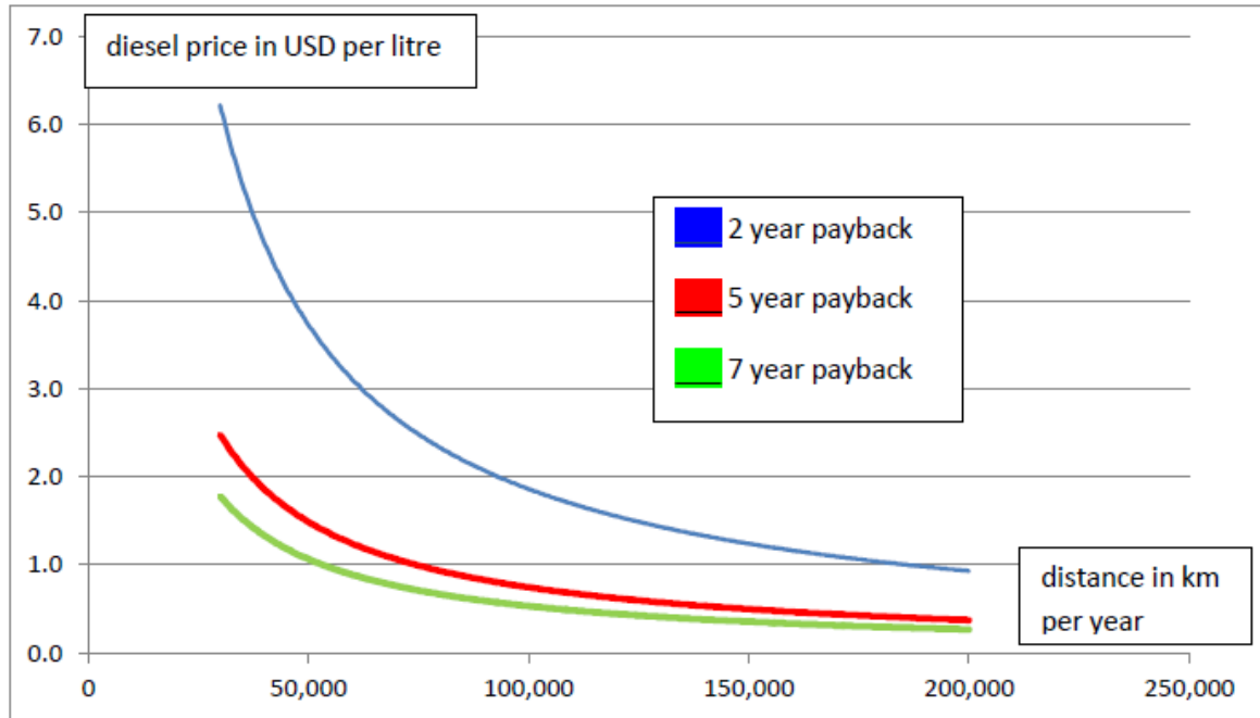
Figure 12: 12m Hybrid-Diesel Constant Payback Combinations of Diesel Price and Distance Driven
