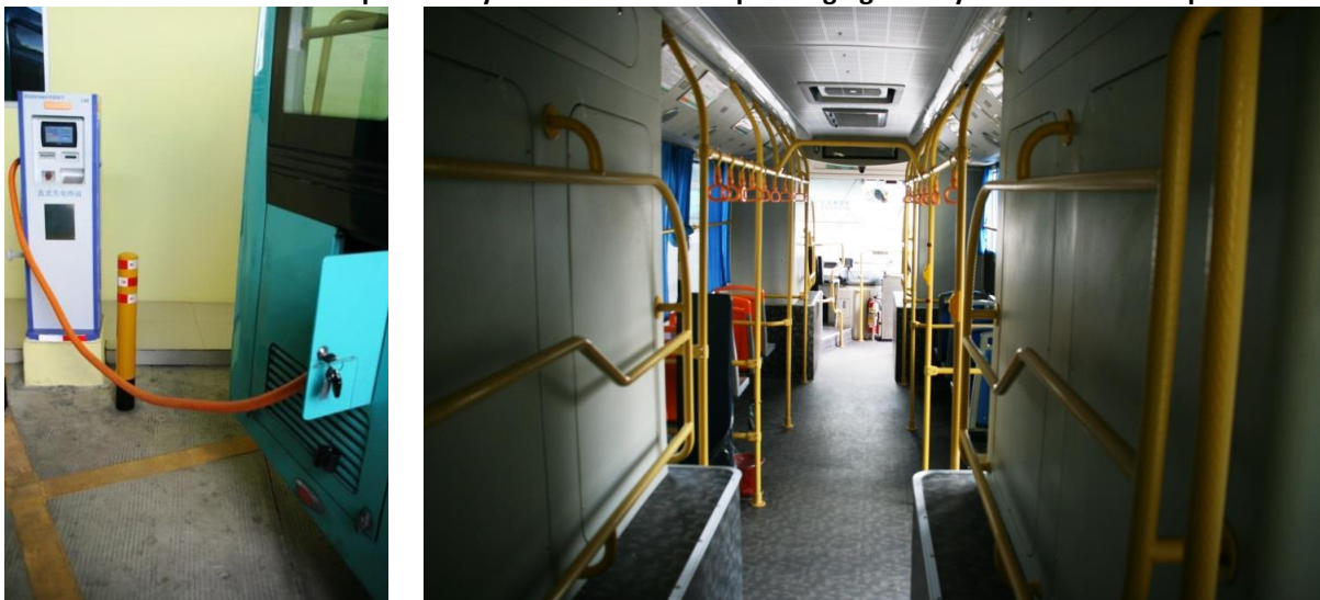
Photo 9: BYD Electric Buses Operated by Shenzhen Bus Group: Charging Facility and Bus Interior Space
