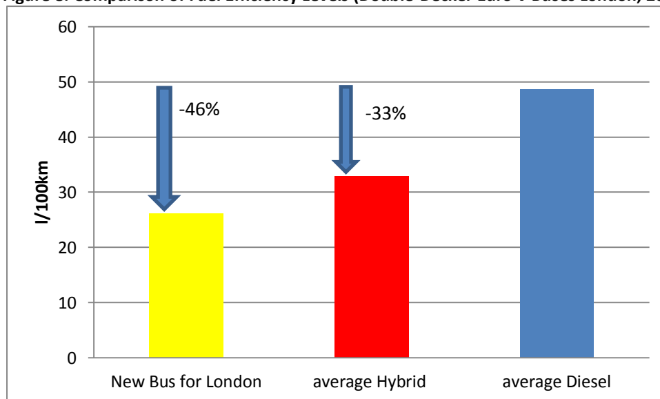
Figure 8: Comparison of Fuel Efficiency Levels (Double-Decker Euro V Buses London, 2013)
