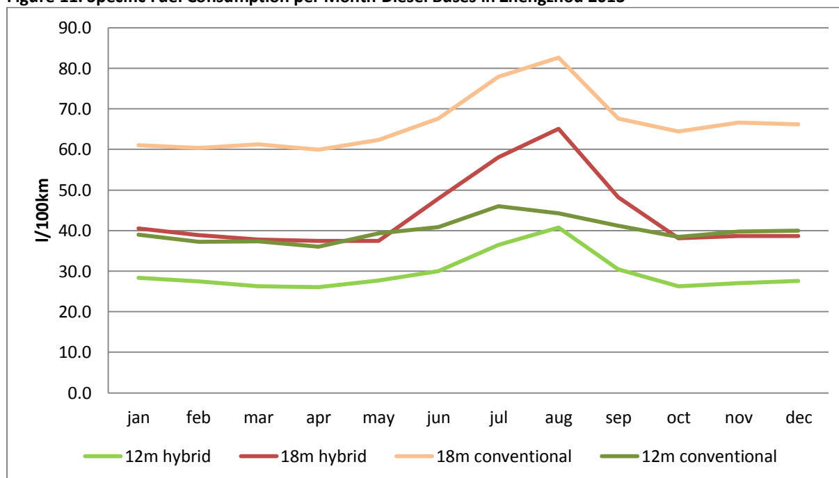
Figure 11: Specific Fuel Consumption per Month Diesel Buses in Zhengzhou 2013
