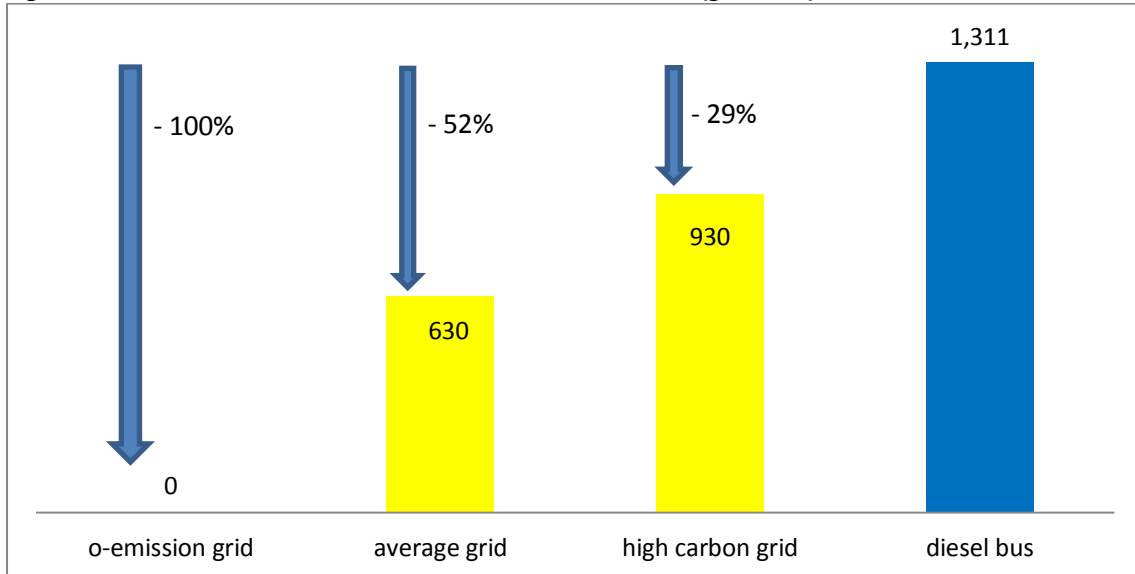
Figure 15: GHG WTW Emissions 12m Electric versus Diesel Bus (gCO 2 /km)
