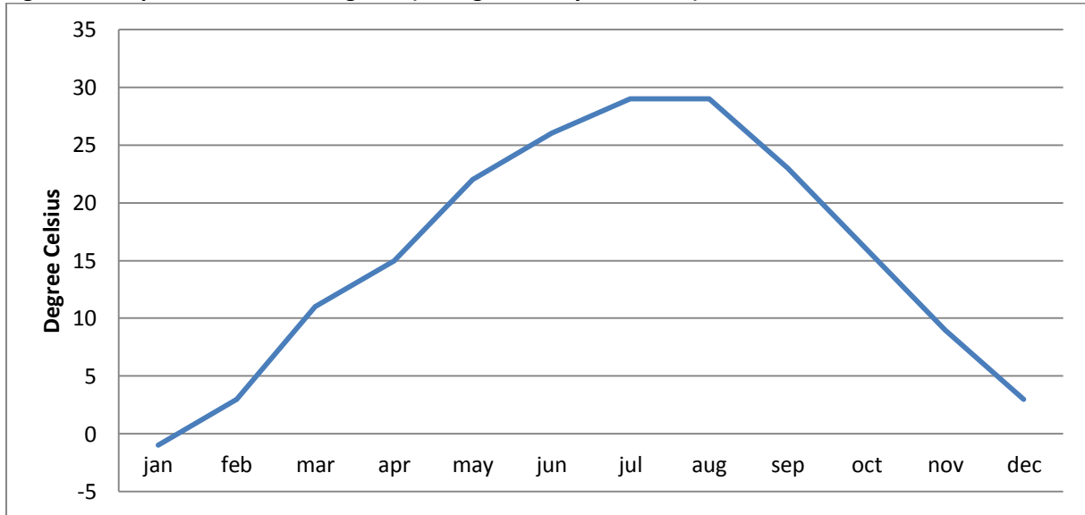
Figure 9: Temperatures 2013 Zhengzhou (average monthly in °Celsius)
