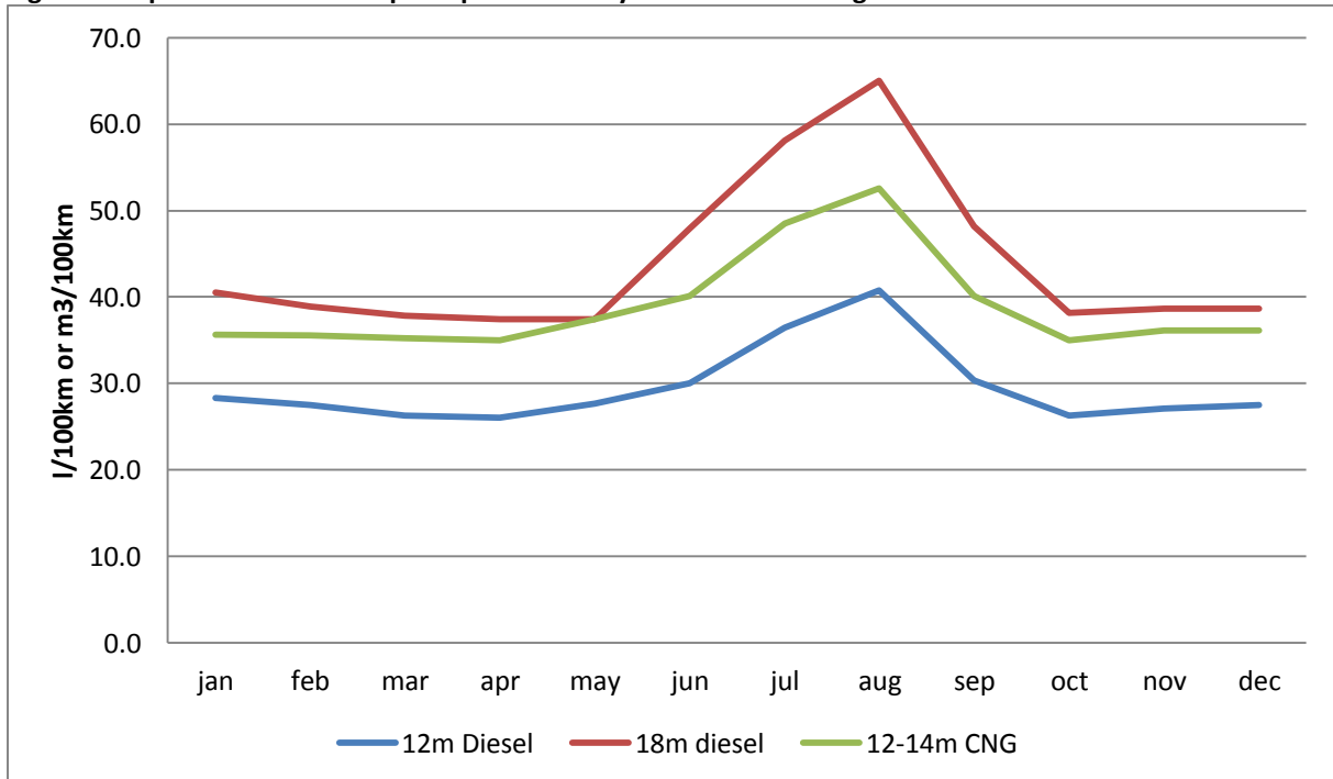
Figure 10: Specific Fuel Consumption per Month Hybrid Buses in Zhengzhou 2013
