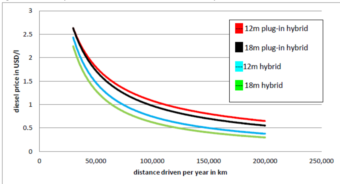
Figure 13: 5-Year Payback Combinations Price/Distance for Diesel Hybrids
